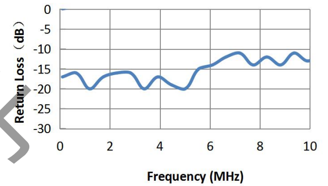
S11
